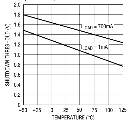
Shutdown Pin Threshold (Off-to-On)
