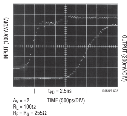
Propagation Delay
