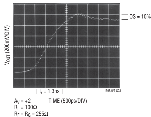
Rise Time and Overshoot
