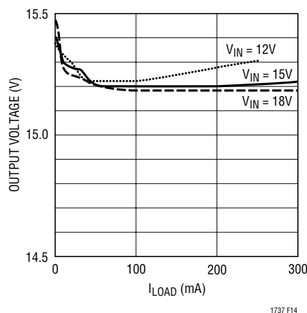
Figure 14. Load Regulation
