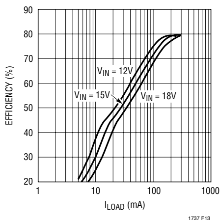
Figure 13. Efficiency vs I_{LOAD}
