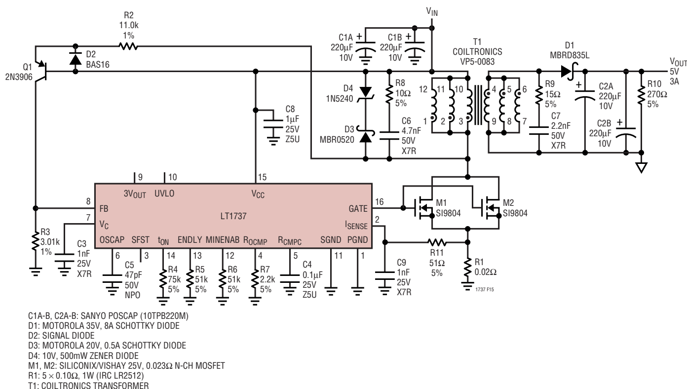
Figure 15. 4.5V-5.5V to Isolated 5V Converter
