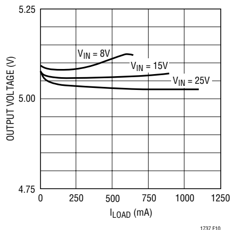
Figure 10. Output Regulation
