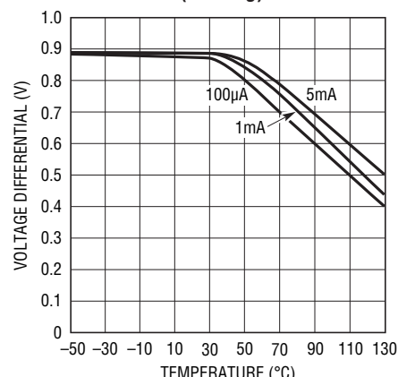
Minimum Input-Output Voltage Differential (Sinking)
