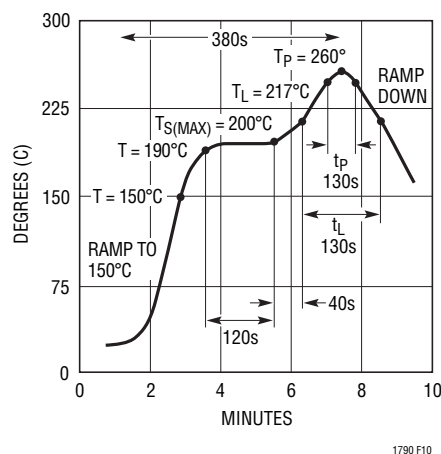
Figure 10. Lead-Free Reflow Profile
