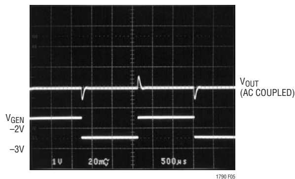
Figure 5. LT1790-2.5 Sourcing 4\text{mA} to 5\text{mA}
