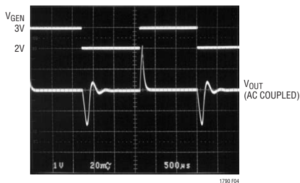
Figure 4. LT1790-2.5 Sourcing and Sinking 0.5\text{mA}
