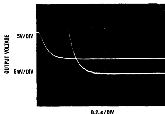
Settling Time
