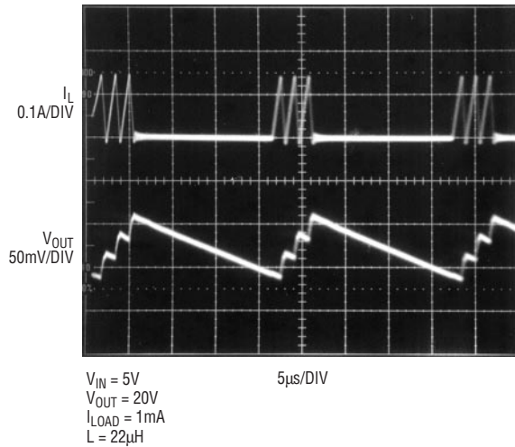
Operating Waveforms
