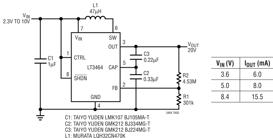
Ultra High Efficiency 20V Output Converter with Output Disconnect
