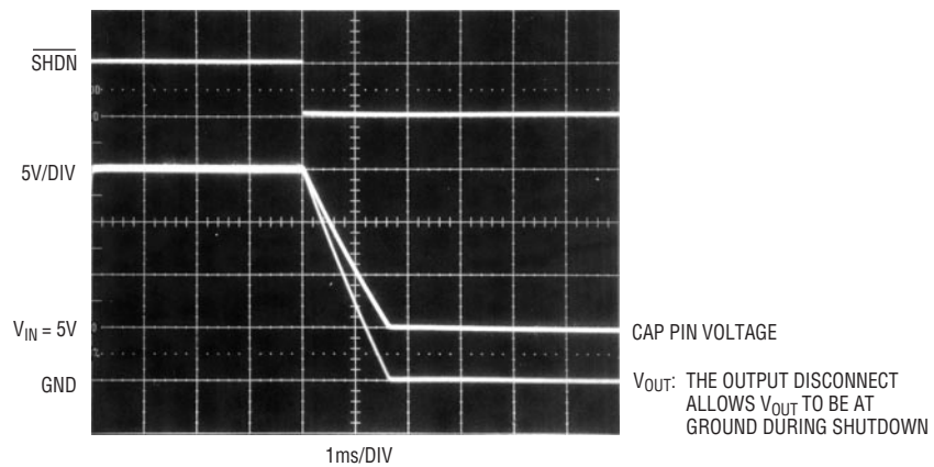
Shutdown Waveforms
