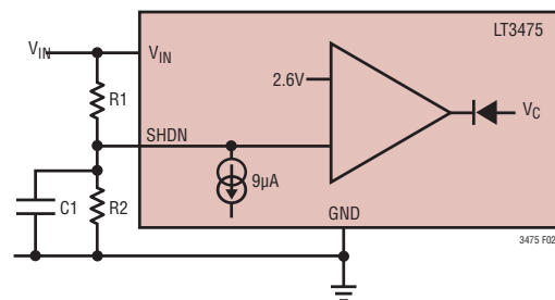
Figure 2. Undervoltage Lockout
