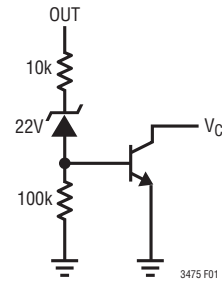
Figure 1. External Overvoltage Protection Circuitry for the LT3475-1
