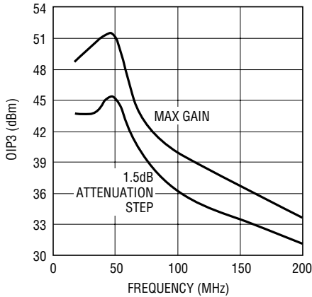
OIP3 vs Frequency at Pin = -23dBm, Max Gain and 1.5dB Attenuation Step, R_{OUT} = 200\Omega
