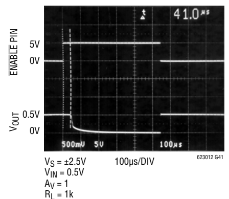
\overline{ENABLE} Pin Response Time
