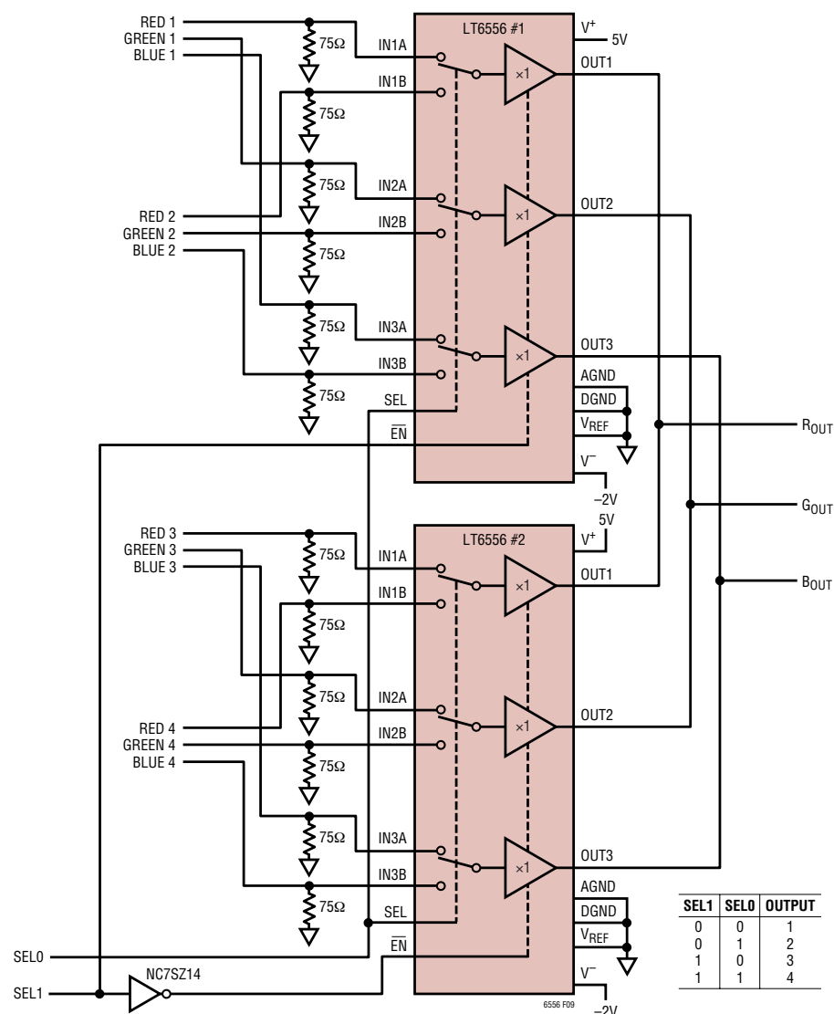
Figure 9. 4:1 RGB Multiplexer
