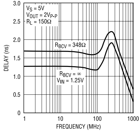
Large-Signal Group Delay
