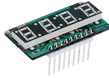
Air Type 7.62mm (.3") Single-In-Line .8"H x 1.6"W x .23"D
