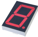
57mm (2.244") Dual-In-Line 1.882"H x 2.744"W x .472"D
