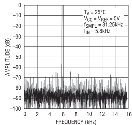
FFT Plot
