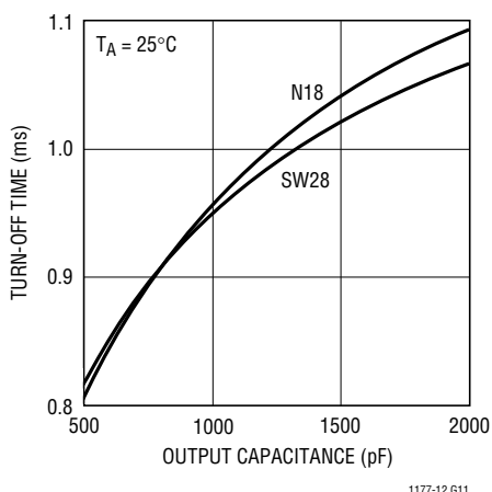
LTC1177-12 Turn-Off Time to V_{OUT} = 1V vs Output Capacitance
