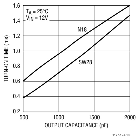
LTC1177-12 Turn-On Time to V_{OUT} = 4.5V vs Output Capacitance
