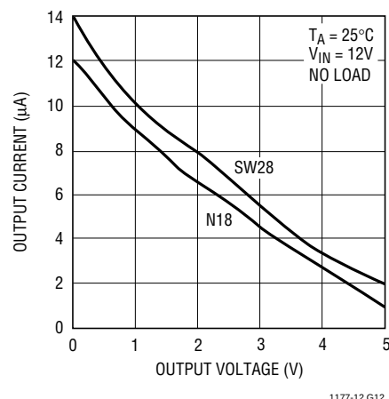
LTC1177-12 Output Current vs Output Voltage
