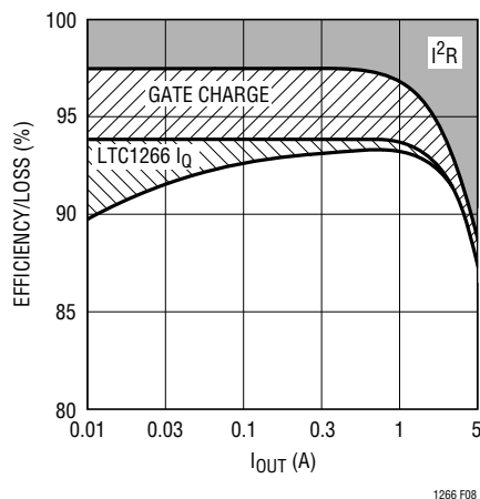
Figure 8. Efficiency Loss
