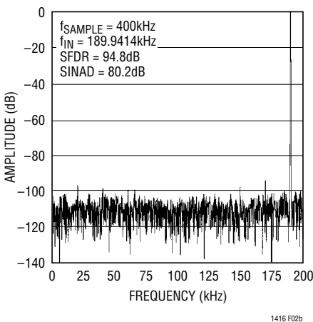
Figure 2b. LTC1416 Nonaveraged, 4096 Point FFT, Input Frequency = 190kHz
