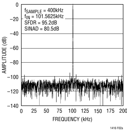
Figure 2a. LTC1416 Nonaveraged, 4096 Point FFT, Input Frequency = 100kHz
