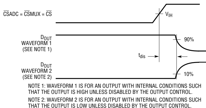
Voltage Waveforms for t_{dis}
