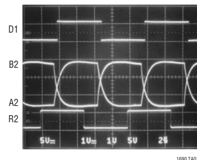
Driving a 1000 Foot STP Cable
