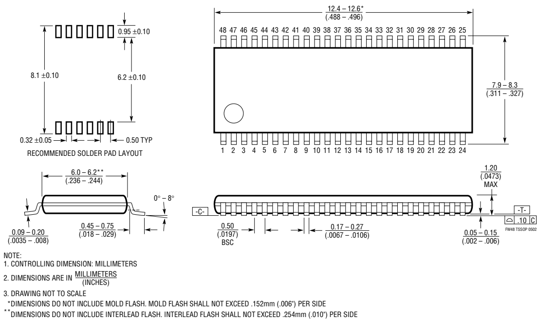
FW Package 48-Lead Plastic TSSOP (6.1mm) (Reference LTC DWG # 05-08-1651)
