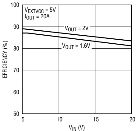
Efficiency vs V_{IN} (Figure 13)
