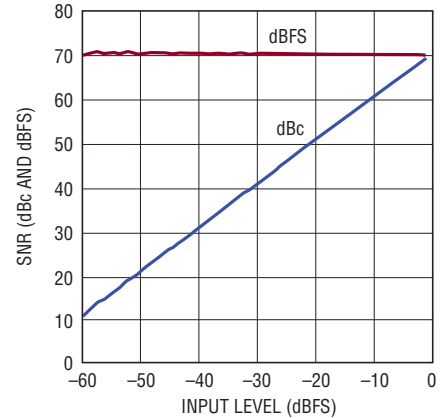
LTC2268-12: SNR vs Input Level, f_{IN} = 70\text{MHz} , 2V Range, 125Msps
