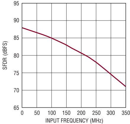
LTC2268-12: SFDR vs Input Frequency, -1dBFS, 2V Range, 125Msps
