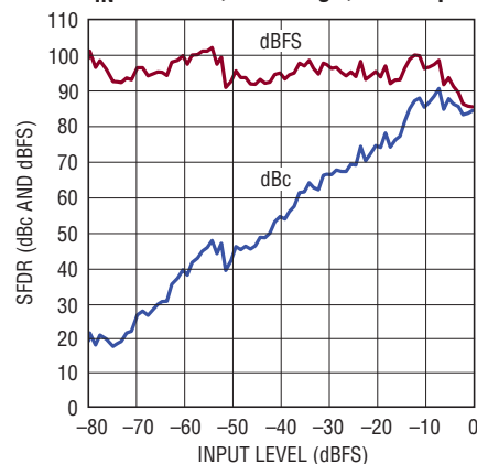
LTC2267-12: SFDR vs Input Level, f_{IN} = 70\text{MHz} , 2\text{V} Range, 105\text{Mps}
