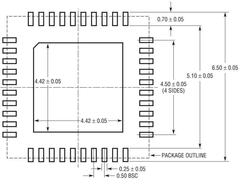
UJ Package 40-Lead (6mm x 6mm) Plastic QFN (Reference LTC DWG # 05-08-1728)
