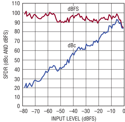
LTC2268-12: SFDR vs Input Level, f_{IN} = 70\text{MHz} , 2V Range, 125Msps
