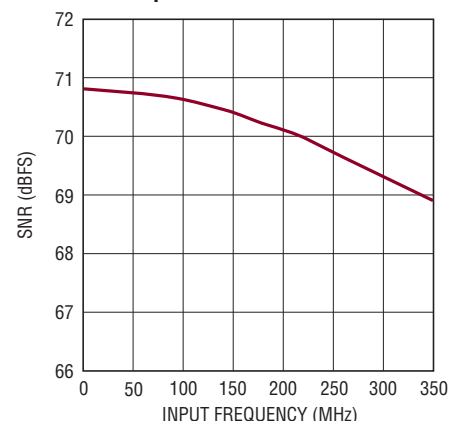
LTC2268-12: SNR vs Input Frequency, -1\text{dBFS} , 2\text{V} Range, 125\text{Msps}
