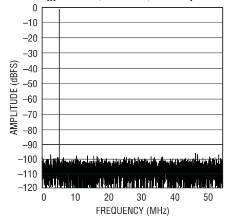
LTC2267-12: 8k Point FFT, f_{IN} = 5\text{MHz} , -1dBFS, 105Msps
