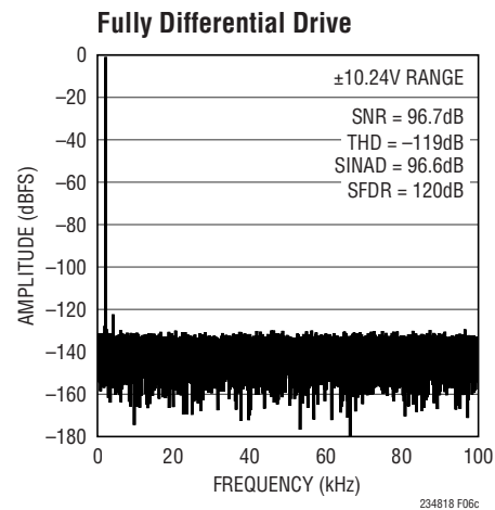
Figure 6c. IN^+/IN^- = -1\text{dBFS} 2kHz Fully Differential Sine, V_{\text{CM}} = 0\text{V} , 32k Point FFT, f_{\text{SAMPL}} = 200\text{ksps} . Circuit Shown in Figure 6a with LT1469 Amplifiers, R_{\text{FILT}} = 49.9\Omega , C_{\text{FILT}} = 1000\text{pF}
