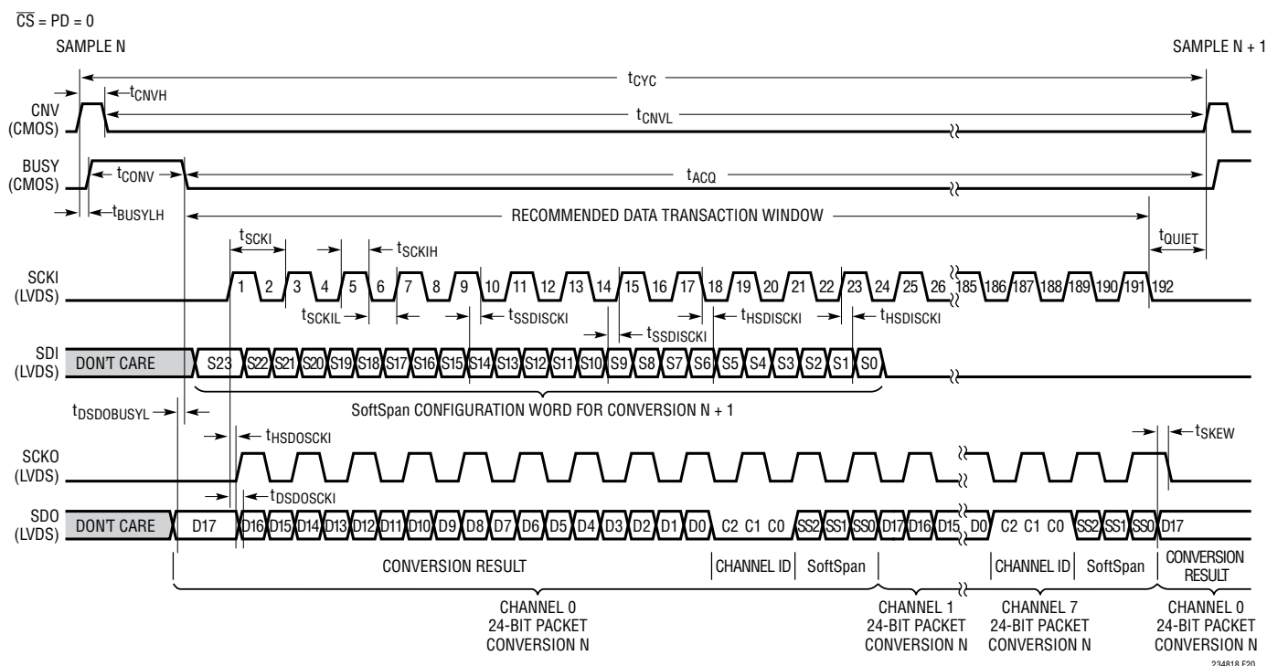
Figure 20. Serial LVDS I/O Mode
