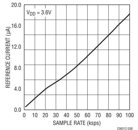
Reference Current vs Sample Rate (TS8 Package)
