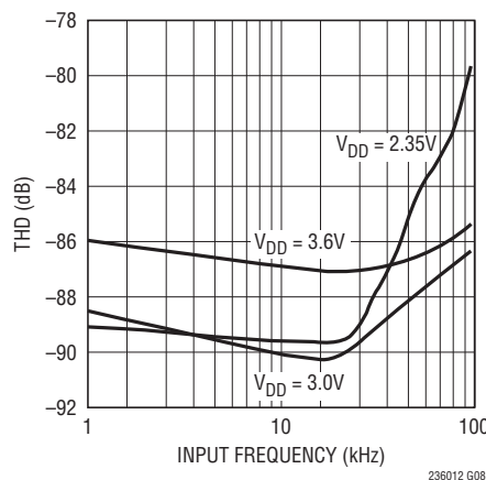
THD vs Input Frequency
