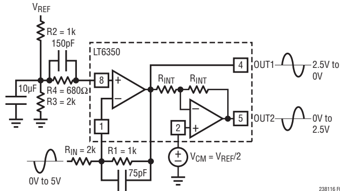
Figure 6. LT6350 Converting a 0V-5V Single-Ended Signal to a \pm 2.5\text{V} Differential Input Signal
