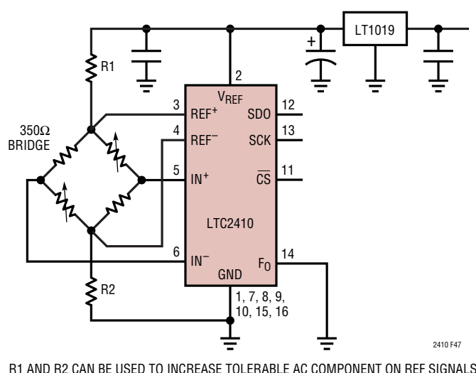
Figure 47. Simple Bridge Connection
