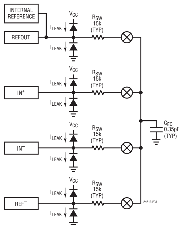
Figure 8. LTC2461/LTC2463 Analog Input/Reference Equivalent Circuit
