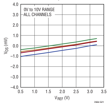
Unipolar Offset vs Reference Input
