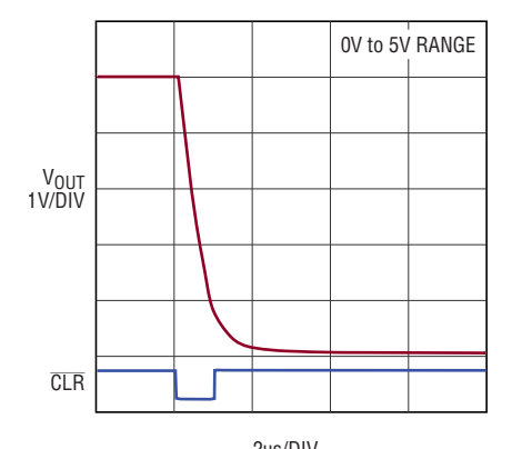
Hardware CLR to Zero-Scale
