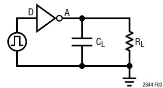
Figure 3. V.10/V.28 Driver Test Circuit
