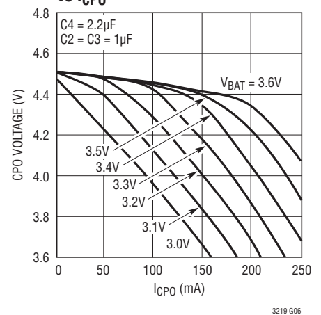
1.5x Mode CPO Voltage vs I_{CPO}
