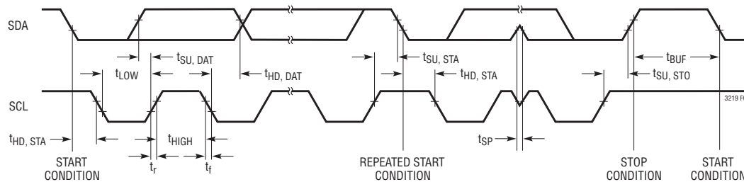
Figure 3. Timing Parameters
