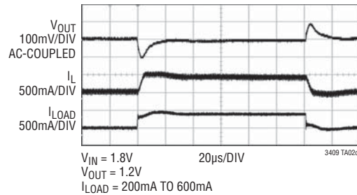
Load Step
