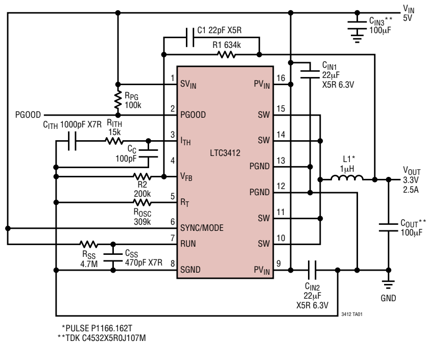
3.3V, 2.5A Step-Down Regulator at 1MHz, Forced Continuous Mode Operation
