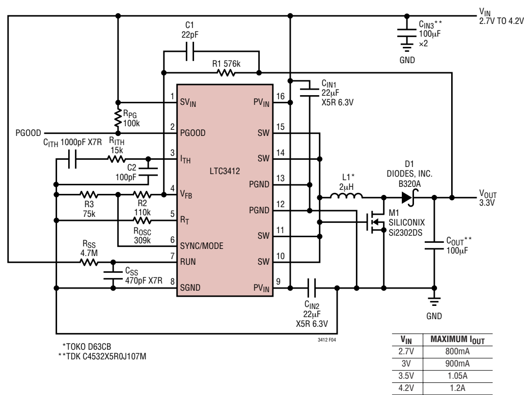
Lithium-Ion to 3.3V, Single Inductor Buck-Boost Converter
