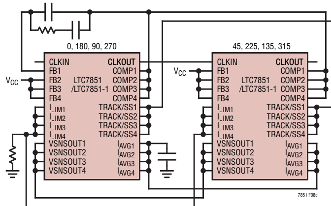
(c) 8-Phase
