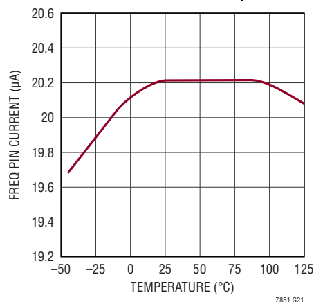
FREQ Pin Current vs Temperature
