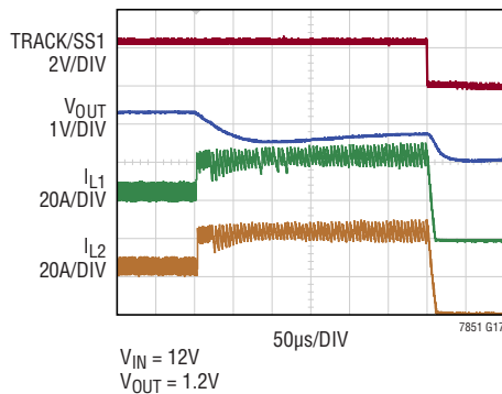
128-Cycle Overcurrent Counter (2-Phase Using FDMF5820DC DrMOS)
