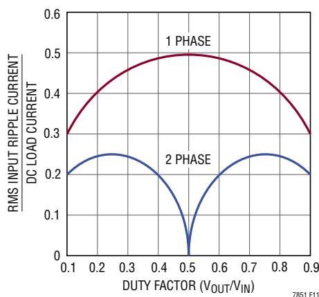
Figure 12. Normalized RMS Input Ripple Current vs Duty Factor for 1 and 2 Output Stages
