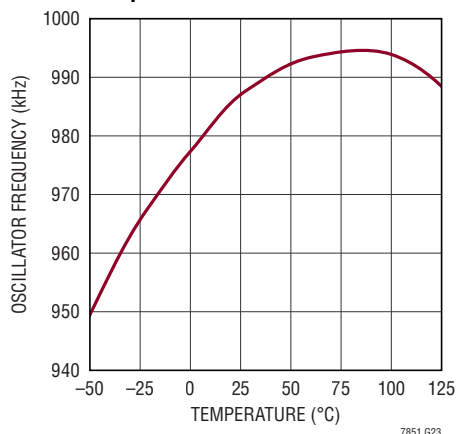
1MHz Preset Frequency vs Temperature
