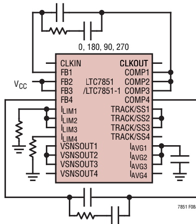
(a) Triple Phase and Single Phase
