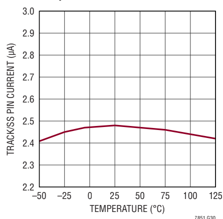
TRACK/SS Pull-Up Current vs Temperature
