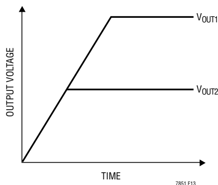
Figure 14. Coincident Tracking
