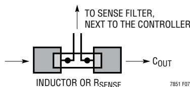
Figure 8. Sense Lines Placement with Inductor or Sense Resistor
