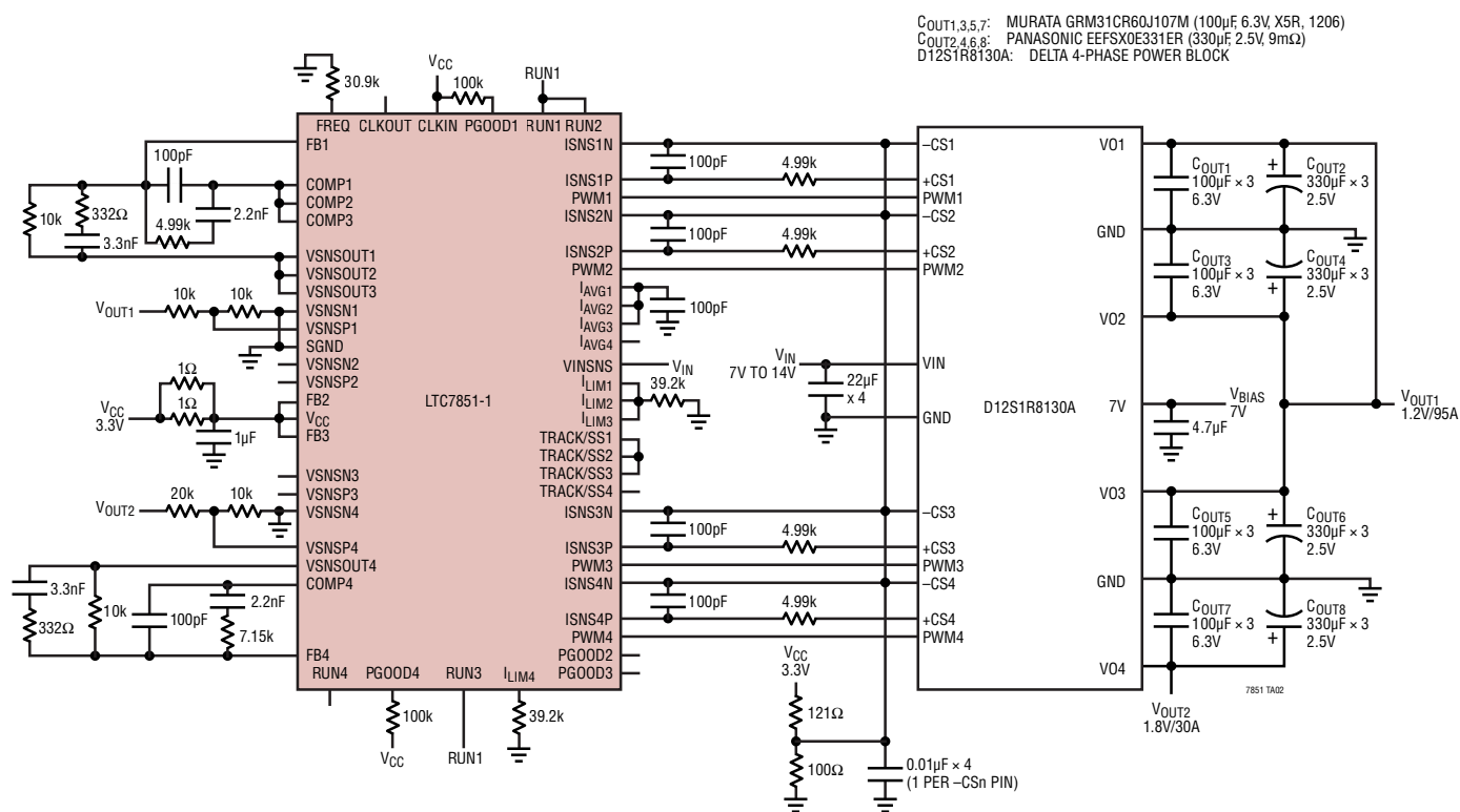
Dual-Output Converter: Triple Phase + Single Phase with Power Block Using the LTC7851-1, f_{sw} = 400\text{kHz}
