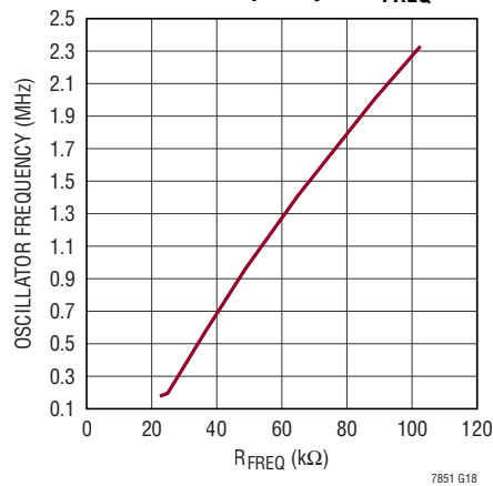
Oscillator Frequency vs R_{FREQ}
