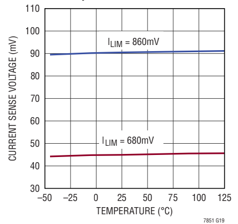
LTC7851-1 Overcurrent Threshold vs Temperature
