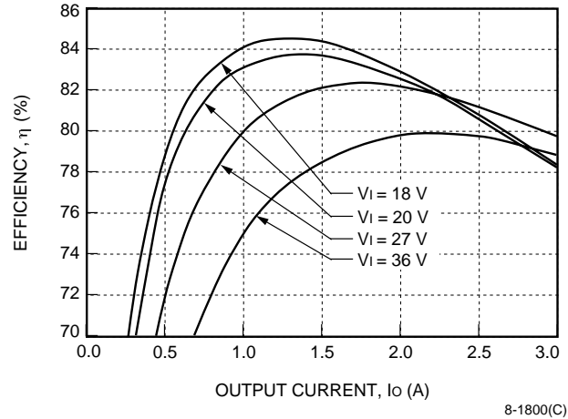
Figure 15. LC015A Typical Efficiency vs. Output Current at T_c = 25\text{ }^\circ\text{C}
