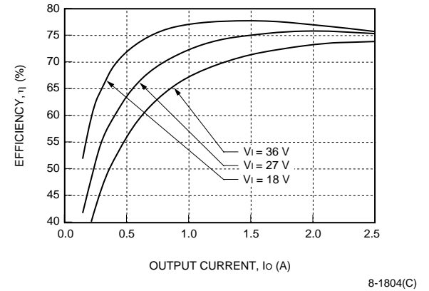
Figure 20. LC010F Typical Efficiency vs. Output Current at T_c = 25\text{ }^\circ\text{C}
