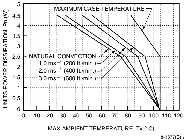
Figure 44. LC015 Forced Convection Power Derating; Either Orientation
