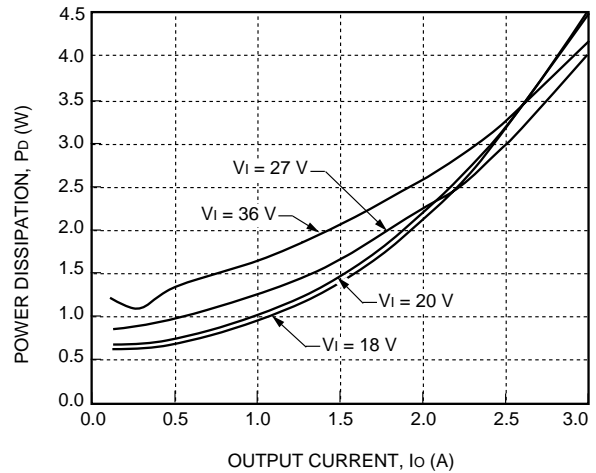
Note: The power dissipation of this unit is shown at T_c = T_{c, max} because the efficiency of this power module drops at high temperatures.
