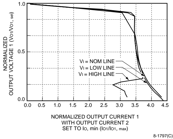
Figure 13. Lx010xx Dual-Output Normalized Output Current vs. Normalized Output Voltage at T_c = 25\text{ }^\circ\text{C} with Other Output at I_{o, \min}
