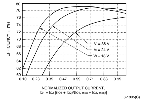
Figure 21. LC010AJ, BK, CL Typical Efficiency vs. Normalized Output Current at T_c = 25\text{ }^\circ\text{C}
