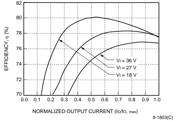
Figure 19. LC010A, B, C Typical Efficiency vs. Normalized Output Current at T_c = 25\text{ }^\circ\text{C}
