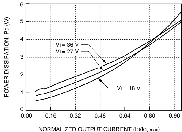
Figure 47. LC015B, C Typical Power Dissipation vs. Normalized Output Current at T_c = 25\text{ }^\circ\text{C}
