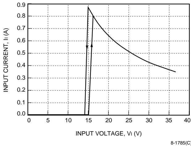
Figure 1. LC010 Input Current vs. Input Voltage at I o = I o, max and T c = 25 °C
