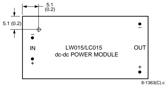
Figure 42. LW015 and LC015 Case Temperature Measurement Location
