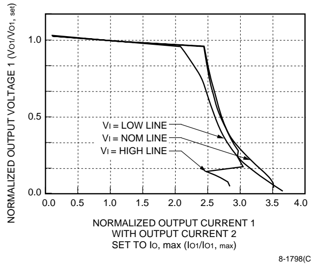
Figure 14. Lx010xx Dual-Output Normalized Output Current vs. Normalized Output Voltage at T_c = 25\text{ }^\circ\text{C} with Other Output at I_o = I_{o, \max}
