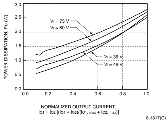
Figure 60. LW010AJ, BK, CL Typical Power Dissipation vs. Normalized Output Current at T_c = 25^\circ\text{C}
