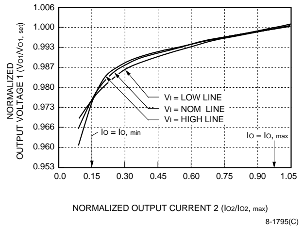
Figure 11. Lx010BK, CL Typical Cross Regulation, Normalized V_{o1} vs. Normalized I_{o2} with Fixed I_{o1} = I_{o, \text{max}} at T_c = 25^\circ\text{C}
