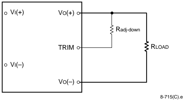
Figure 39. Circuit Configuration to Decrease Output Voltage
