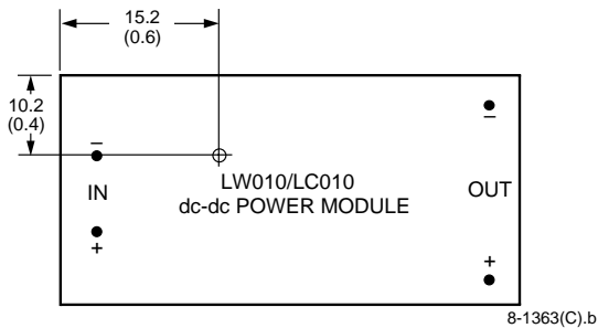
Figure 41. LW010 and LC010 Case Temperature Measurement Location
