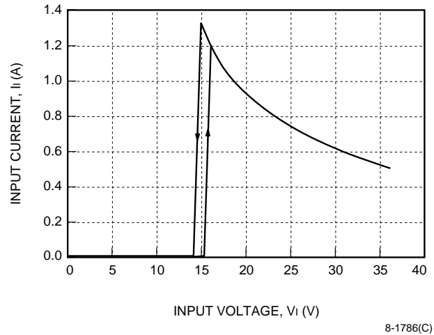
Figure 2. LC015 Input Current vs. Input Voltage at I o = I o, max and T c = 25 °C
