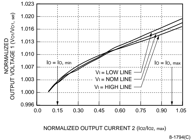
Figure 10. Lx010BK, CL Typical Cross Regulation, Normalized V_{o1} vs. Normalized I_{o2} with Fixed I_{o1} = I_{o, \text{min}} at T_c = 25^\circ\text{C}
