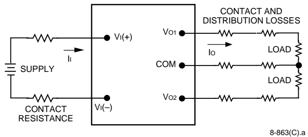
Figure 36. Peak-to-Peak Output Noise Measurement Test Setup for Dual Outputs
