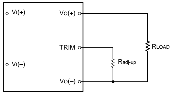
Figure 40. Circuit Configuration to Increase Output Voltage
