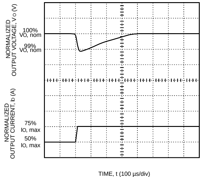
Figure 8. LW020A, B, C, F, and G Typical Output Voltage for a Step Load Change from 50% to 75%
