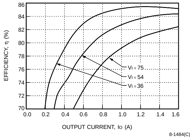
Figure 6. LW020B Typical Converter Efficiency vs. Output Current, T_A = 25^\circ\text{C}
