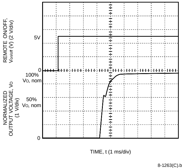
Figure 10. LW020A, B, C, F, and G Typical Output Voltage Start-Up when Signal Applied to Remote On/Off
