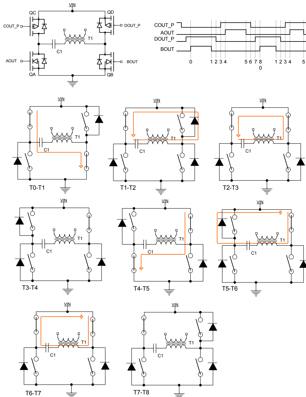
Figure 2 – State Diagram
