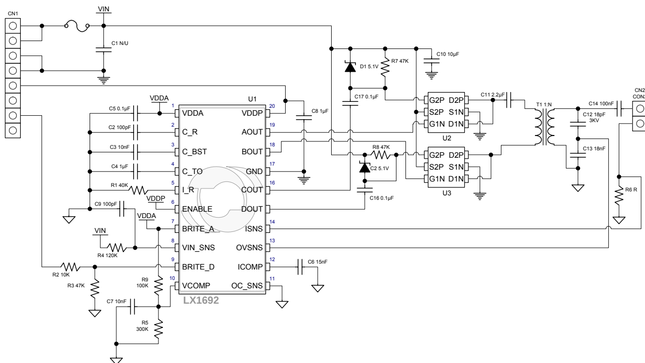
Figure 3 – Schematic
