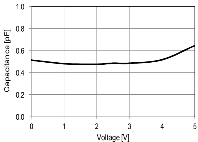
Voltage—Capacitance Characteristic
