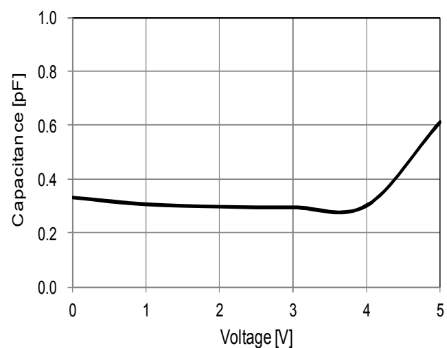
Voltage—Capacitance Characteristic
