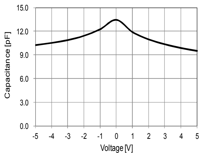
Voltage—Capacitance Characteristic
