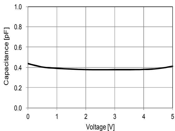
Voltage—Capacitance Characteristic
