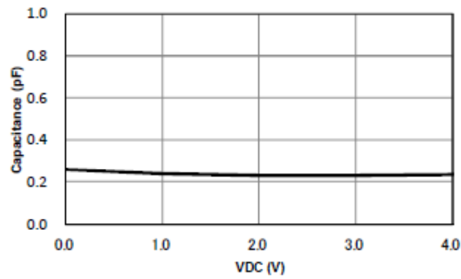
Voltage—Capacitance Characteristic
