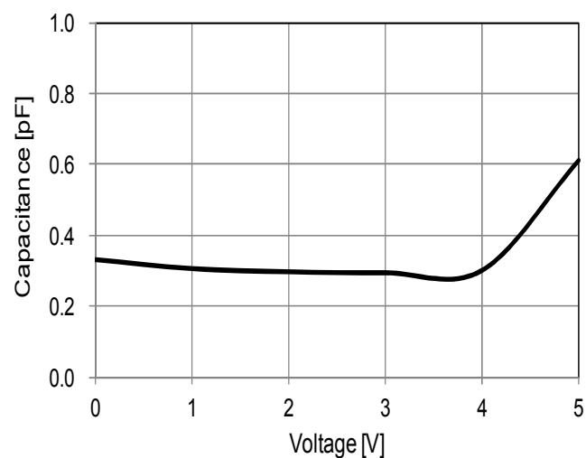
Voltage — Capacitance Characteristic
