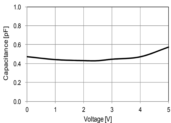
Voltage—Capacitance Characteristic
