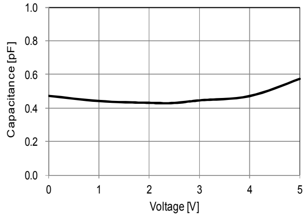
Voltage—Capacitance Characteristic
