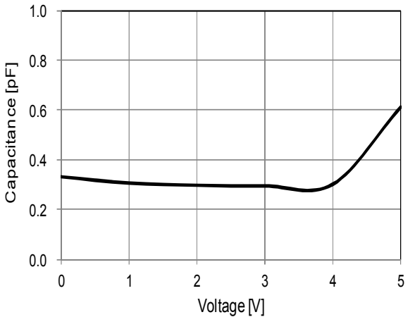
Voltage—Capacitance Characteristic
