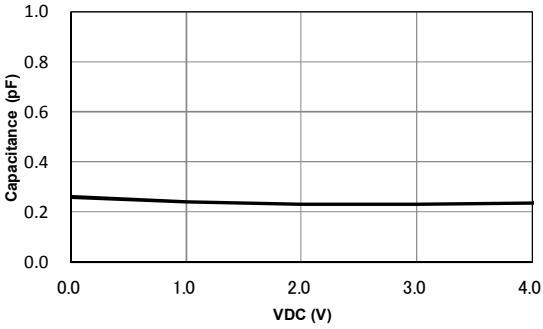
Voltage—Capacitance Characteristic
