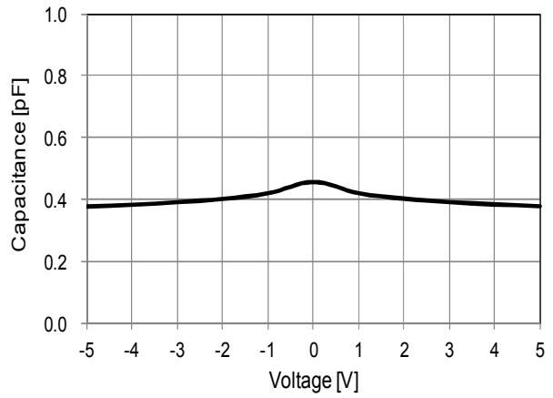
Voltage—Capacitance Characteristic
