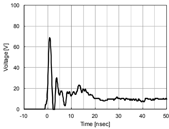
ESD Waveform(IEC61000-4-2:8kV Contact)
