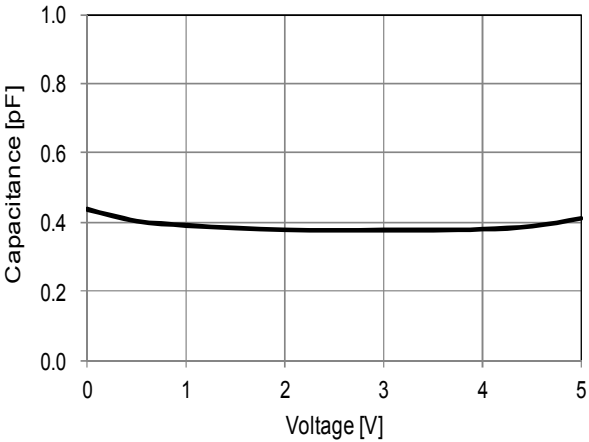
Voltage—Capacitance Characteristic
