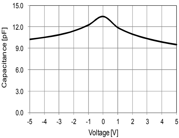
Voltage—Capacitance Characteristic
