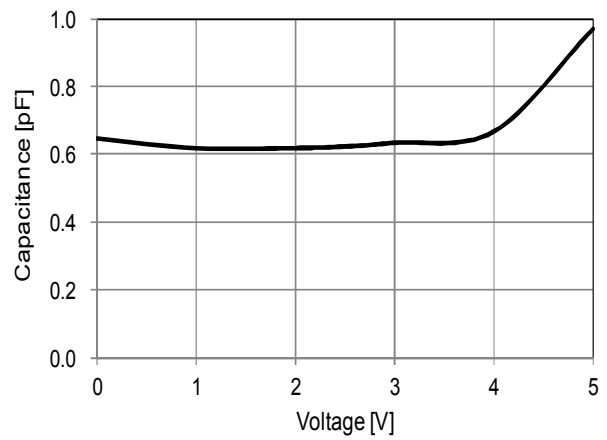
Voltage — Capacitance Characteristic
