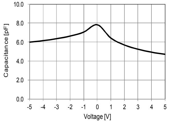
Voltage—Capacitance Characteristic
