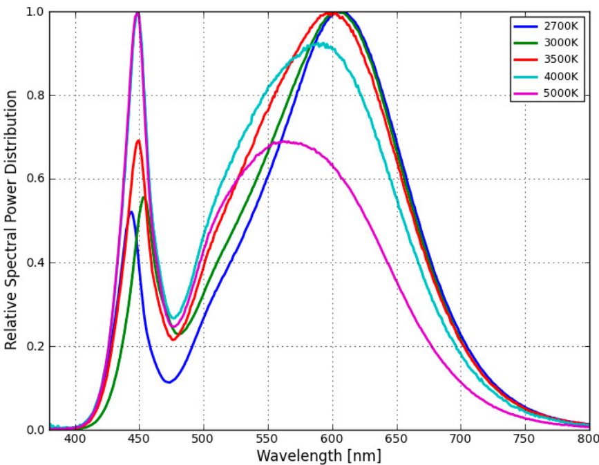
Figure 8. Color spectrum of 80 minimum CRI integrated measurement.
