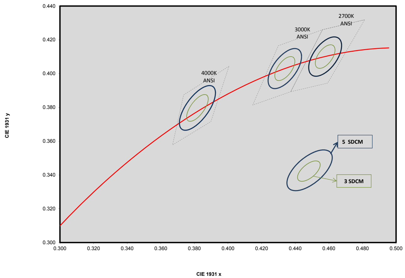
Figure 21. LUXEON H 2700K, 3000K, and 4000K 3-step and 5-step MacAdam ellipse color definition.
