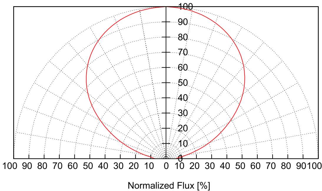
Figure 13. Typical polar radiation pattern for LUXEON H White 4 emitter (LXV8-PWxx-x0x4).
