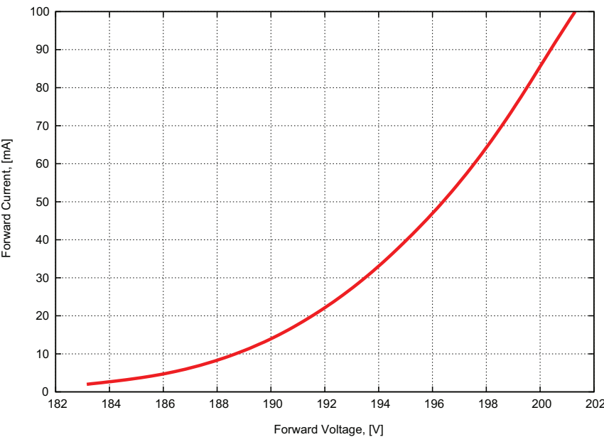
Figure 10. Forward voltage vs. forward current, applicable to LXV8-PWxx-x02x.
