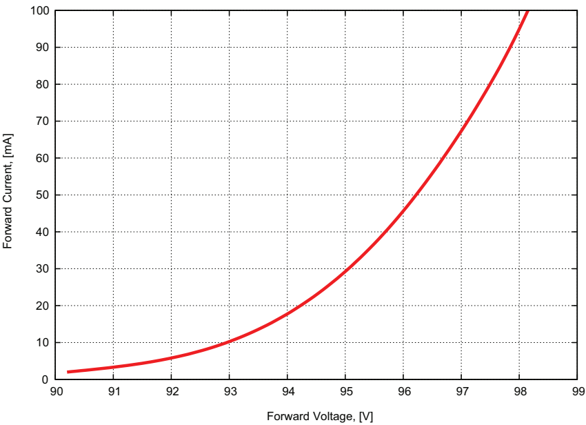
Figure 9. Forward voltage vs. forward current, applicable to LXV8-PWxx-x01x.
