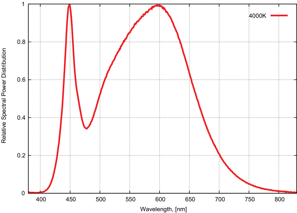
Figure 4. Color spectrum of LXV8-PW40-x0xx, 4000K emitters, integrated measurement.
