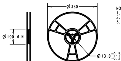
REEL DETAILS
