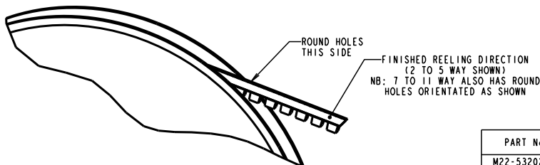
REEL DETAILS
