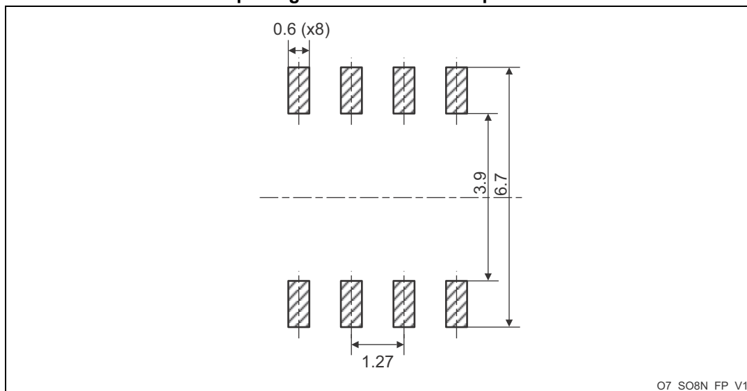
Figure 14. SO8N – 3.9x4.9 mm, 8-lead plastic small outline, 150 mils body width, package recommended footprint
