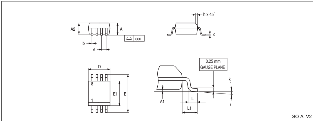
Figure 13. SO8N – 3.9x4.9 mm, 8-lead plastic small outline, 150 mils body width, package outline
