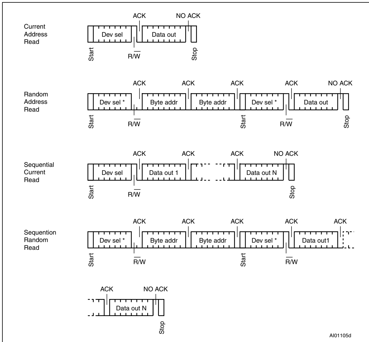
Figure 8. Read mode sequences
