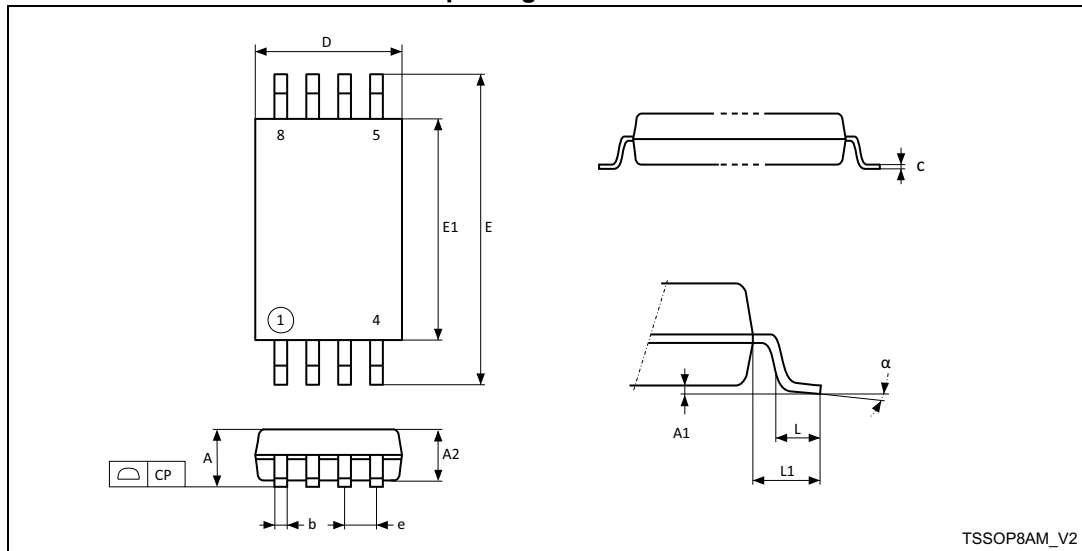
Figure 12. TSSOP8 – 3x4.4 mm, 0.65 mm pitch, 8-lead thin shrink small outline, package outline
