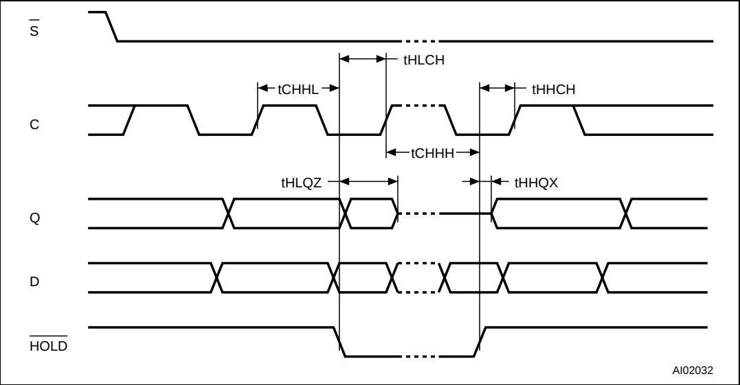
Figure 24. Hold Timing
