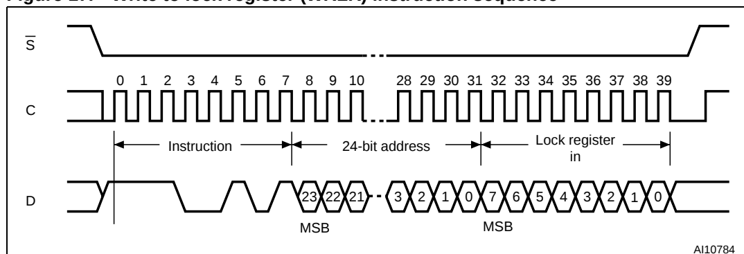
Figure 17. Write to lock register (WRLR) instruction sequence
