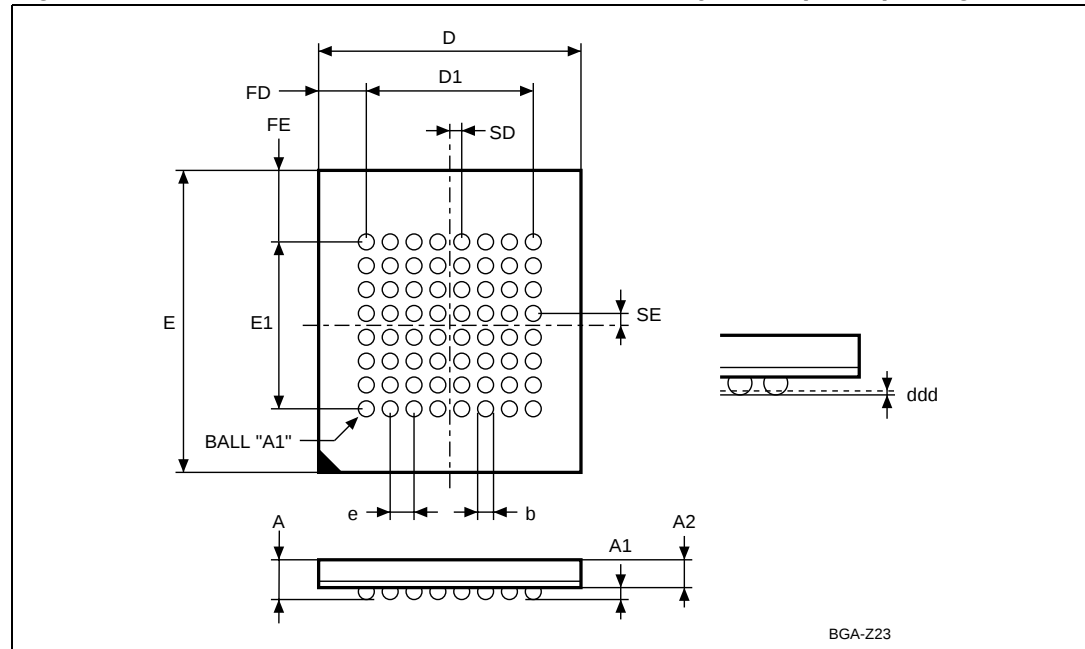
Figure 29. LBGA64 11 x 13 mm—8 x 8 active ball array, 1 mm pitch, package outline
