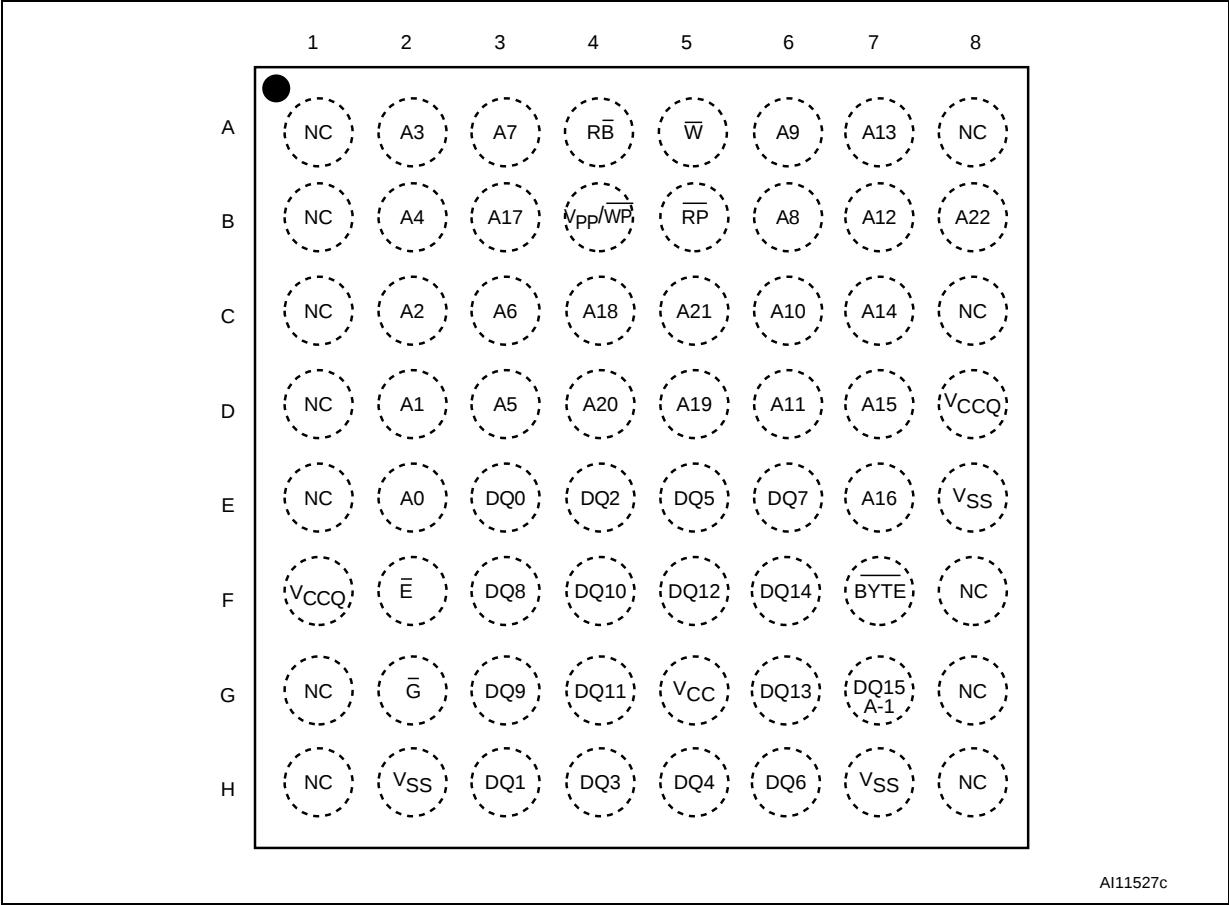
Figure 3. TBGA and LBGA connections (top view through package)
