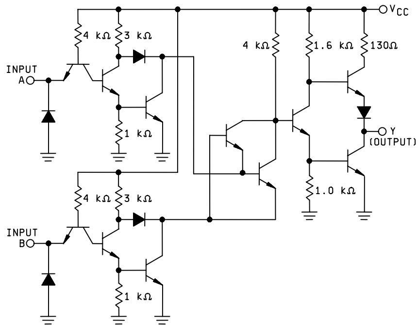
CIRCUIT A
