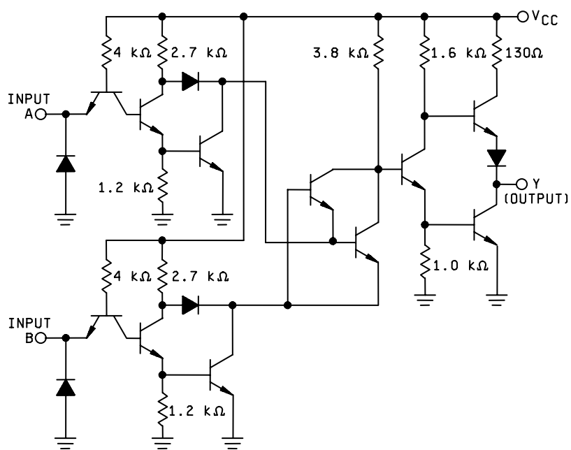
CIRCUIT D
