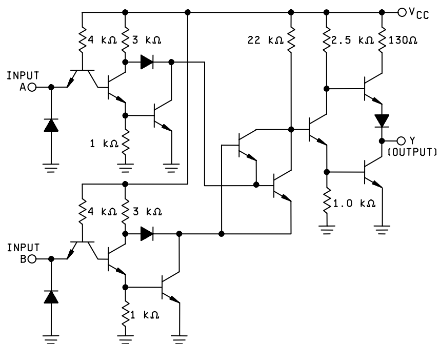
CIRCUIT B
