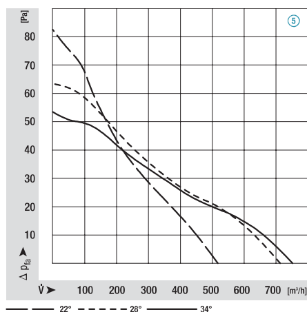
M4Q045-CA03-**, Ø 230, 50 Hz
