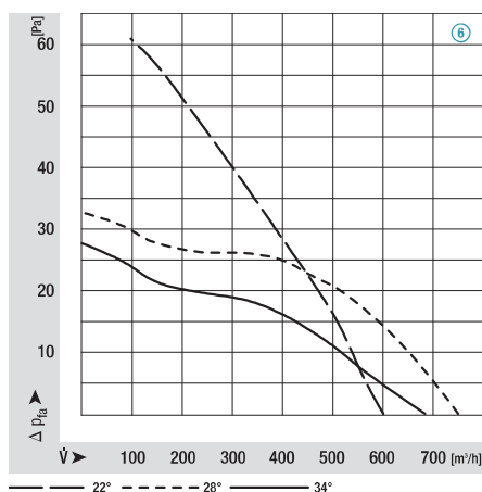
M4Q045-CA03-**, Ø 230, 60 Hz
