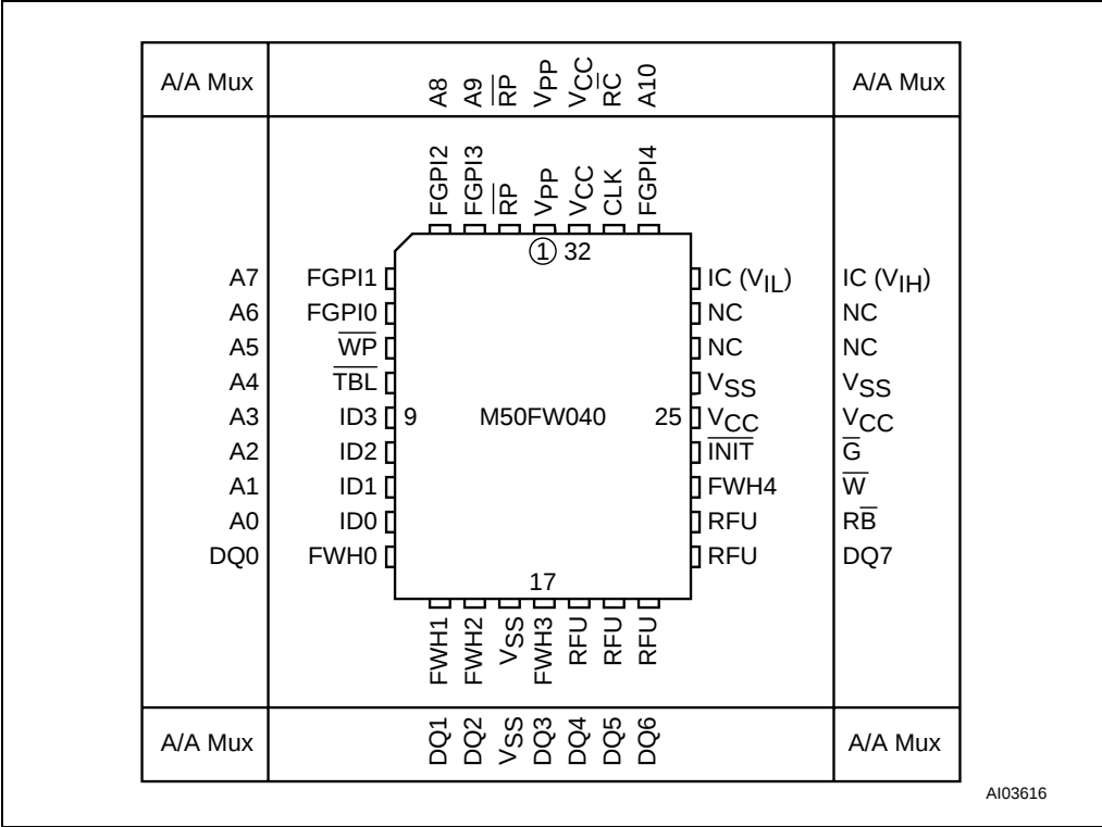
Figure 3. PLCC connections
