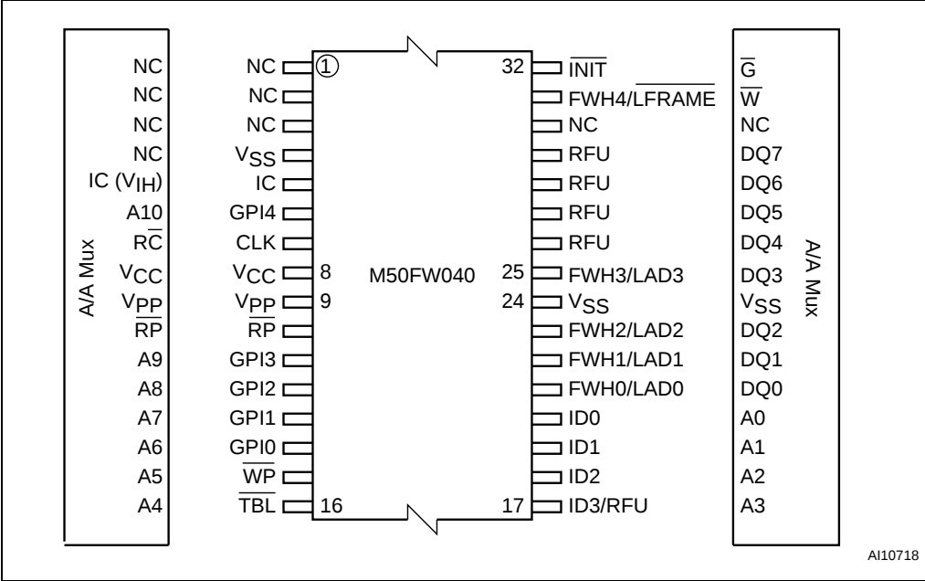
Figure 4. TSOP32 connections
