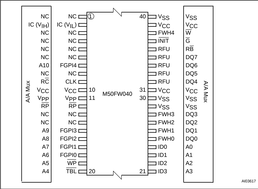
Figure 5. TSOP40 connections
