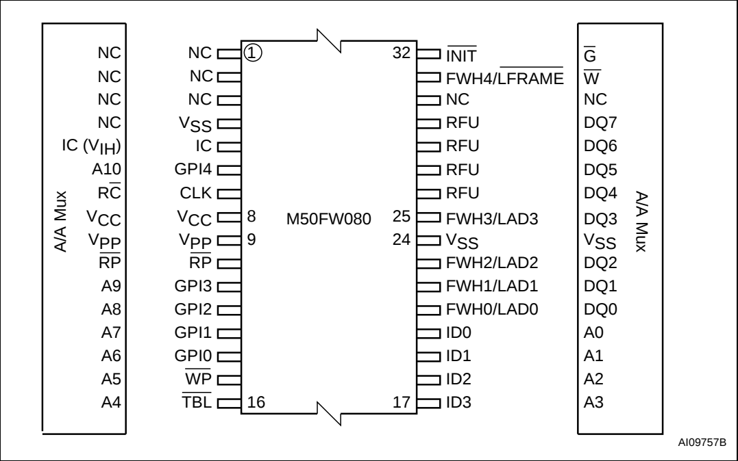
Figure 4. TSOP32 connections
