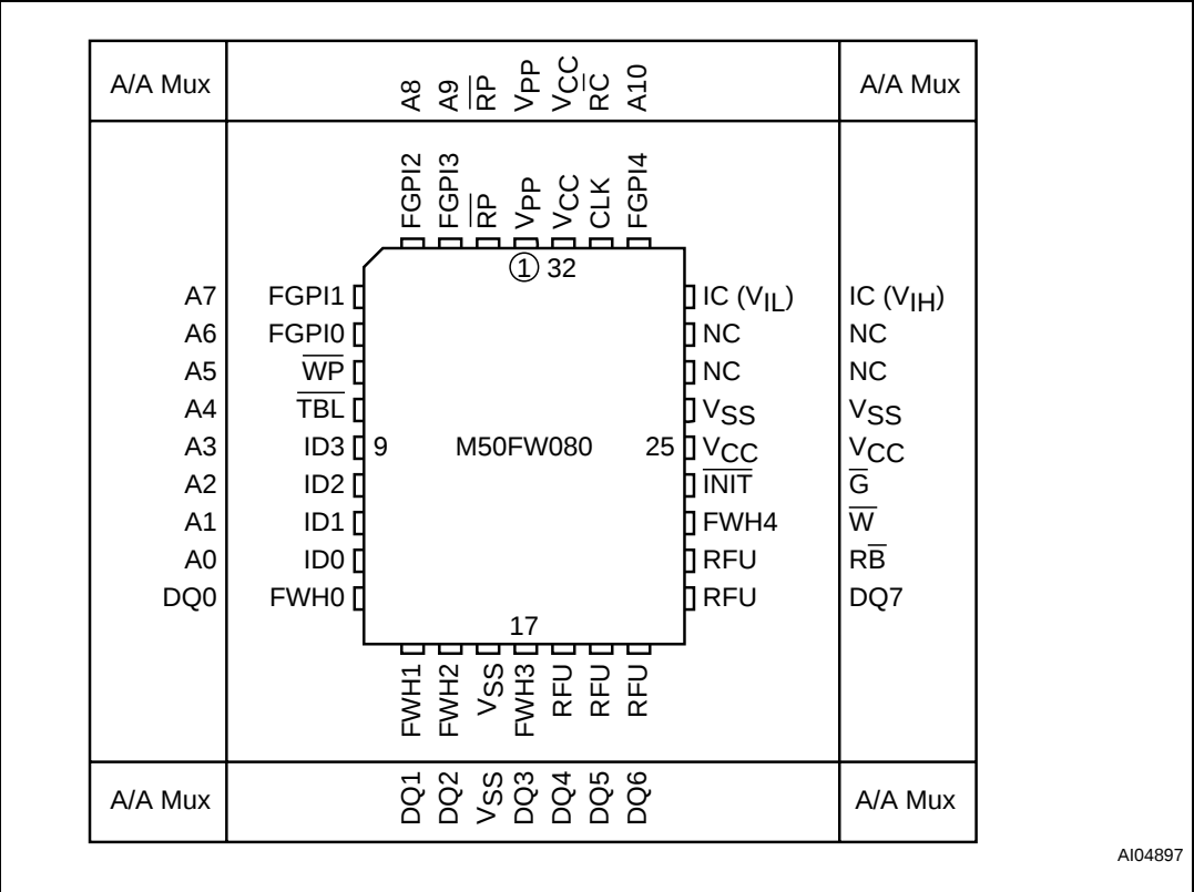
Figure 3. PLCC connections
