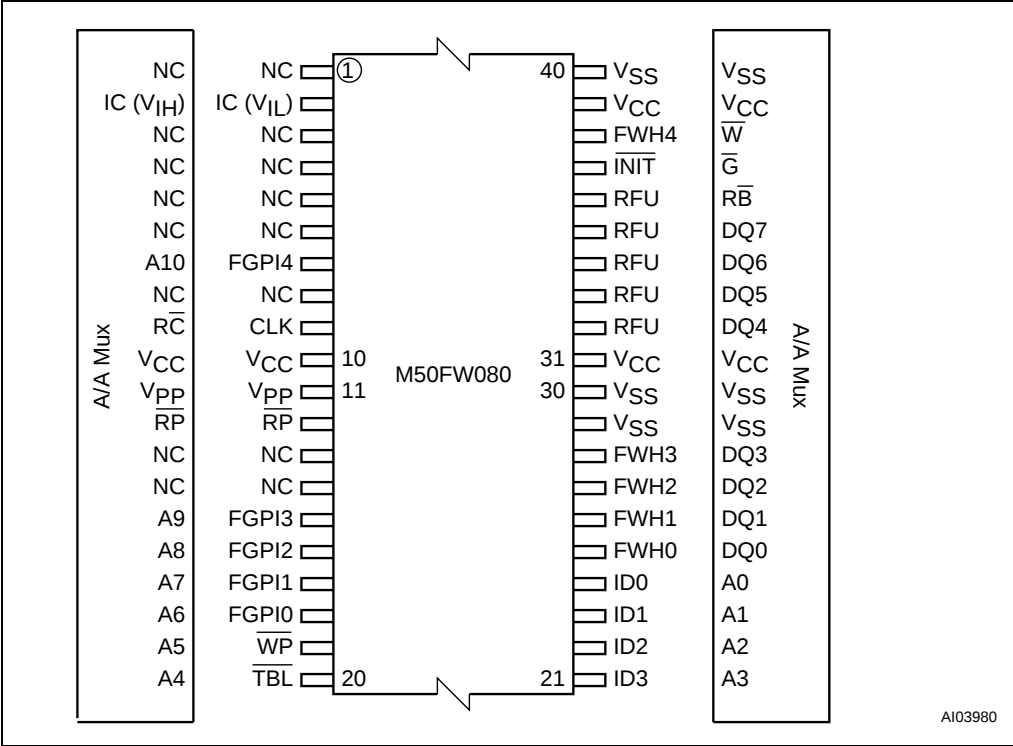
Figure 5. TSOP40 connections
