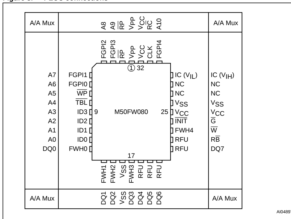
Figure 3. PLCC connections
