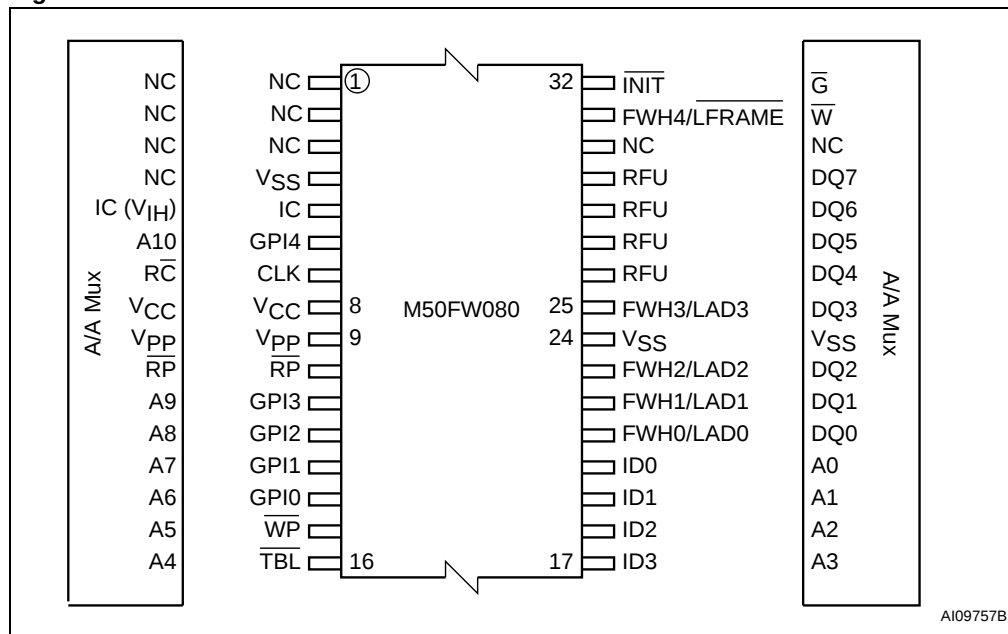
Figure 4. TSOP32 connections
